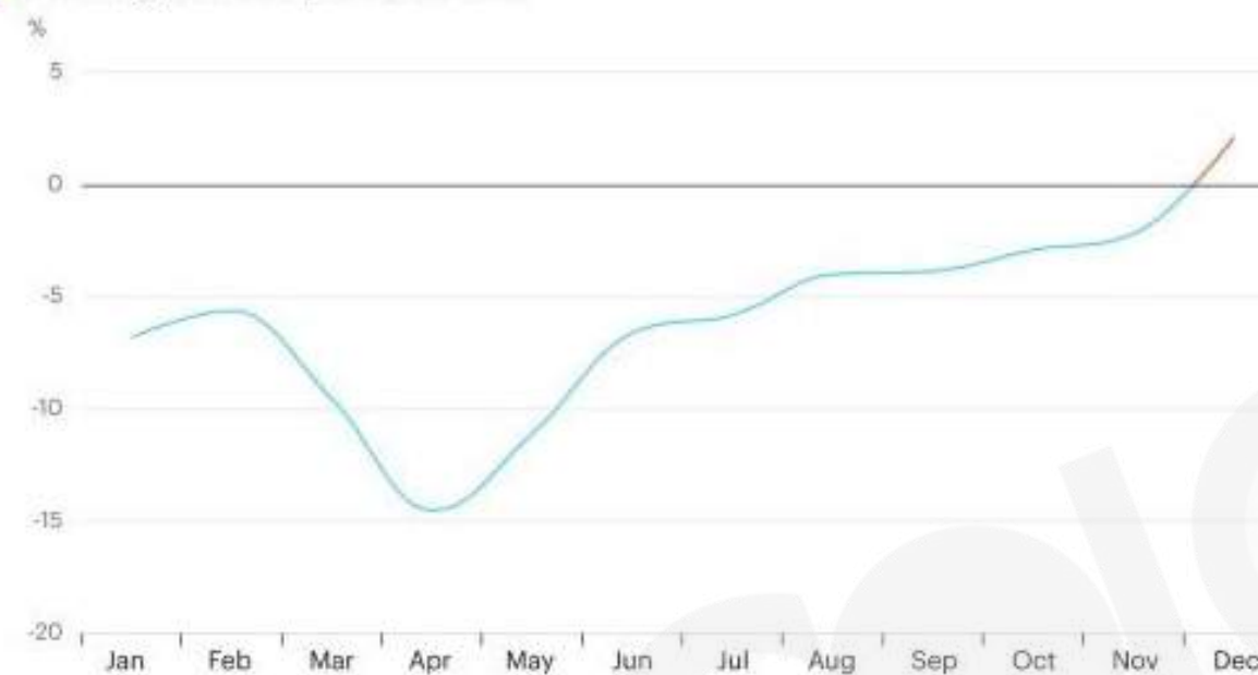
Monthly evolution of global CO 2 emissions, 2020 relative to 2019 Global Energy Review: CO 2 Emissions in 2020
